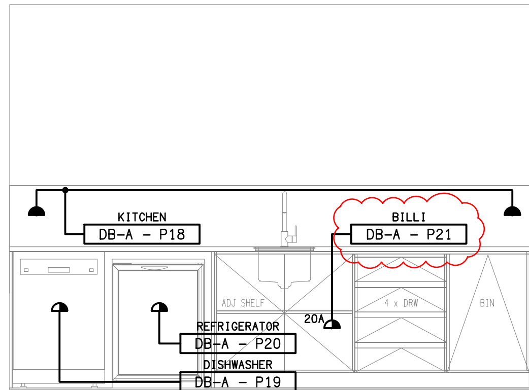
DETAIL A MITSUBISHI KITCHENETTE ELEVATION SCALE 1:25
