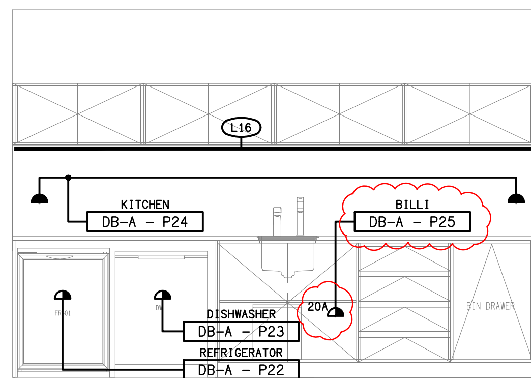
DETAIL B KIA KITCHENETTE ELEVATION SCALE 1:25
